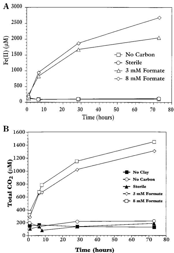
FIGURE 1. (A) Respiration of structural Fe(III) in smectite by MR-1 in a minimal medium with clay added as the sole electron acceptor and formate added as the sole electron donor. (B) Production of \Sigma\text{CO}_2 in the same duplicate MR-1 cultures. Smectite was added to 7.5 \text{ g L}^{-1} . Each value is the average calculated from duplicate cultures and measurements ranged less than 5% from the average of duplicates.
